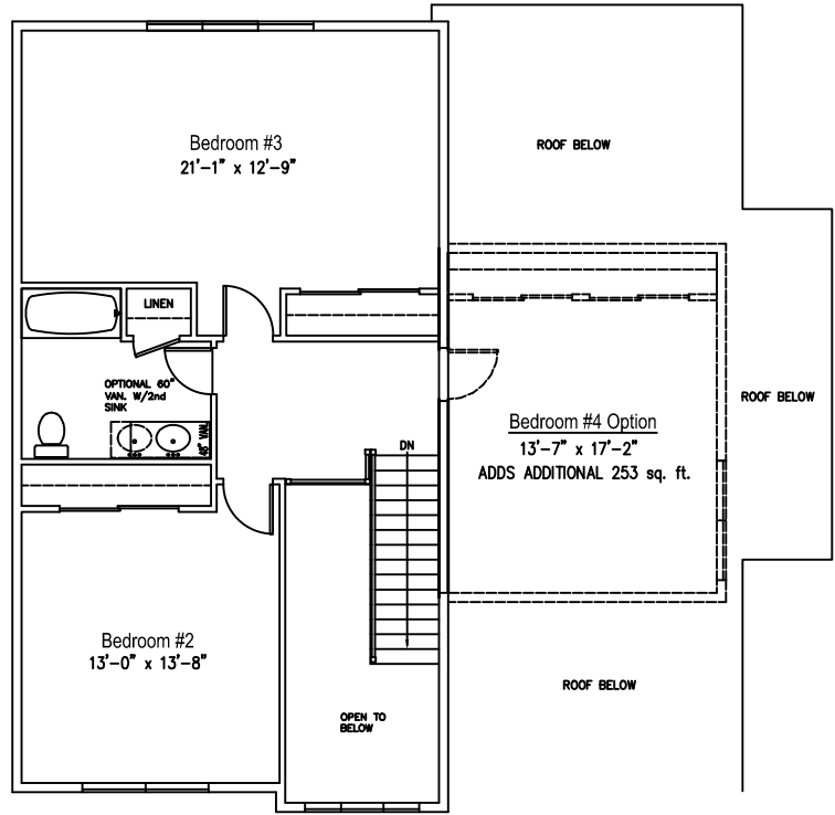
LONGFELLOW 1 SECOND FLOOR
