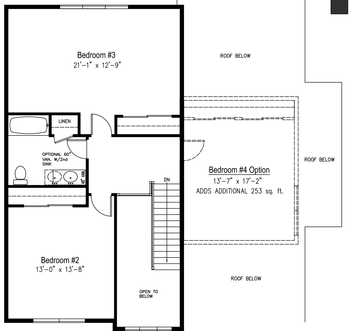
LONGFELLOW I SECOND FLOOR
