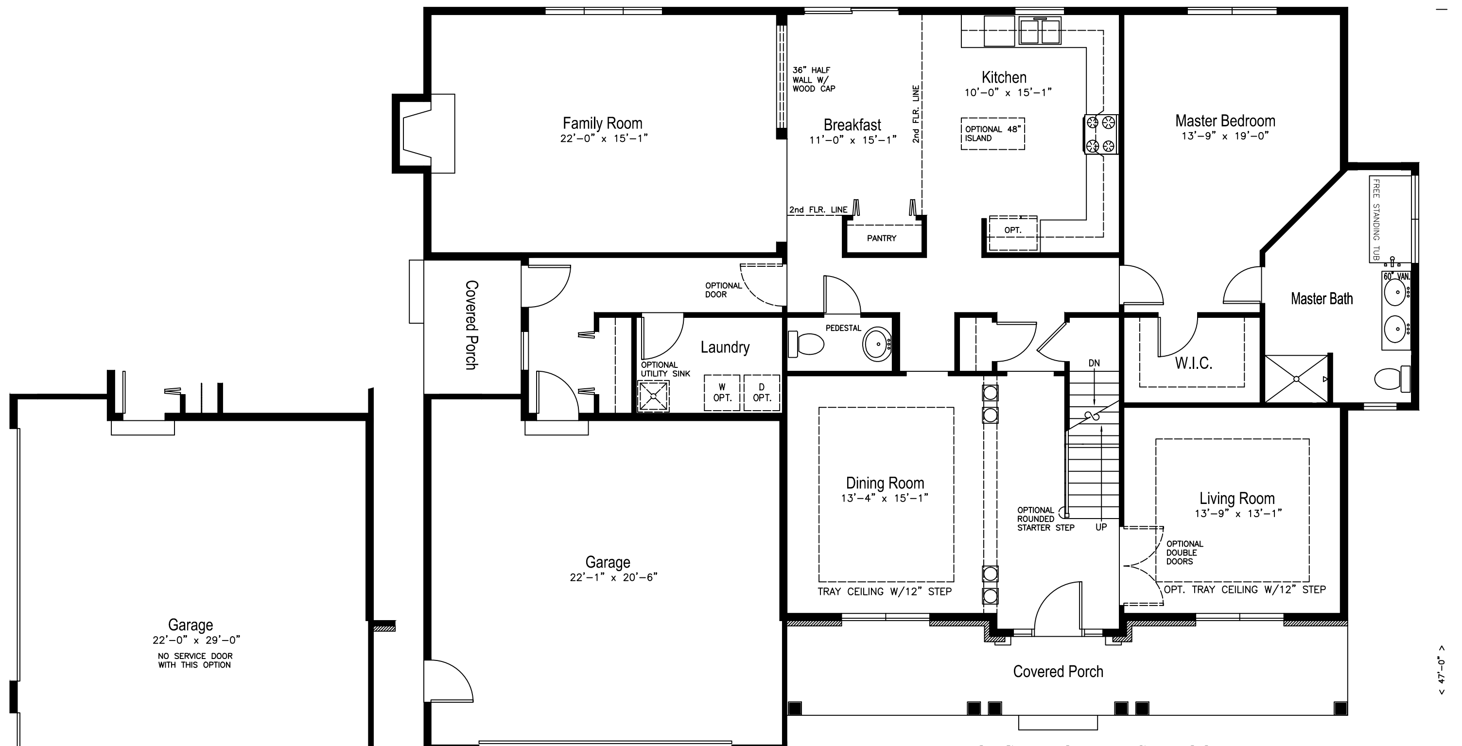
LONGFELLOW I FIRST FLOOR
