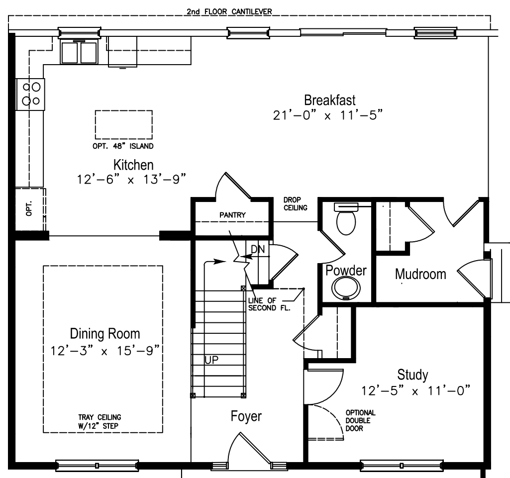
Optional Open First Floor Plan
