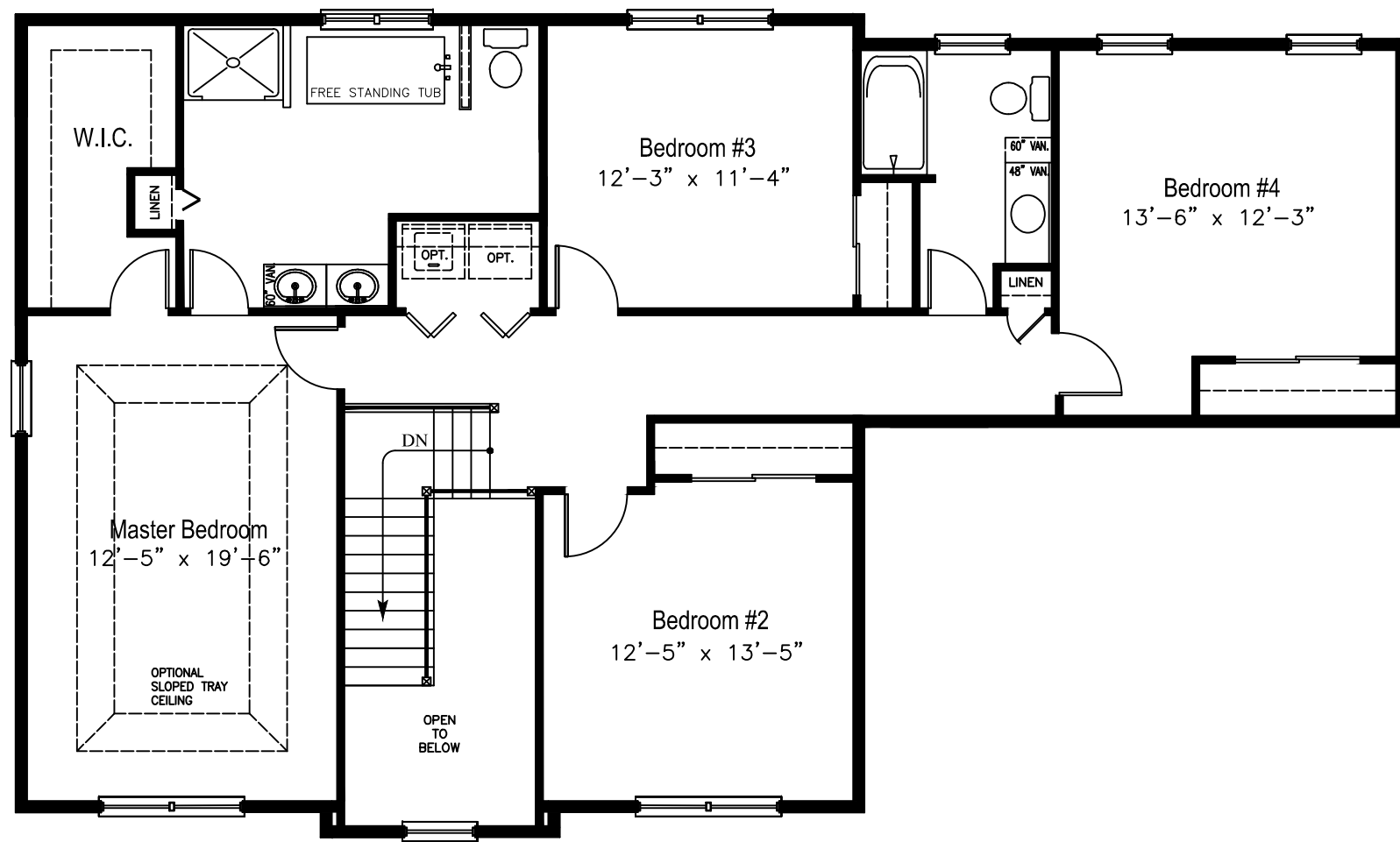
EMERSON II SECOND FLOOR
