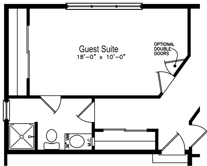
Guest Suite Option ADDITIONAL 142.0 sq. ft.
