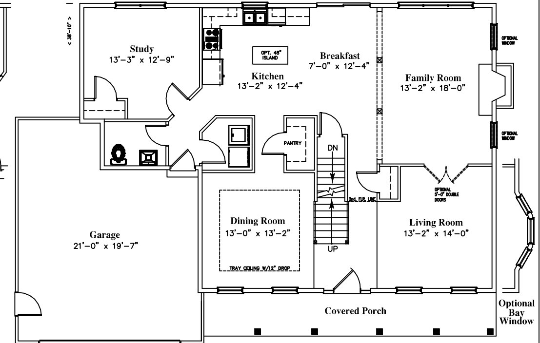
BRENTWOOD 2 FIRST FLOOR
