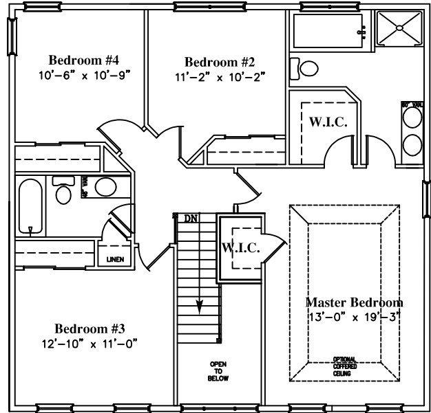
BRENTWOOD 2 SECOND FLOOR
