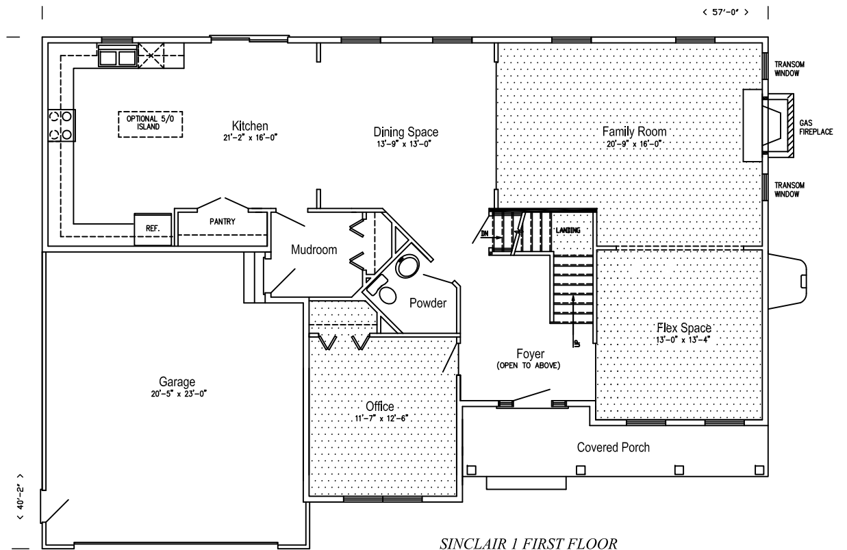
SINCLAIR 1 FIRST FLOOR
