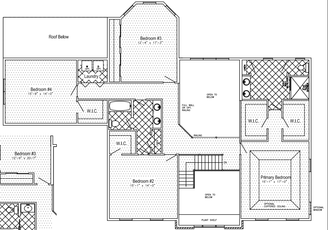
HEMINGWAY SECOND FLOOR
