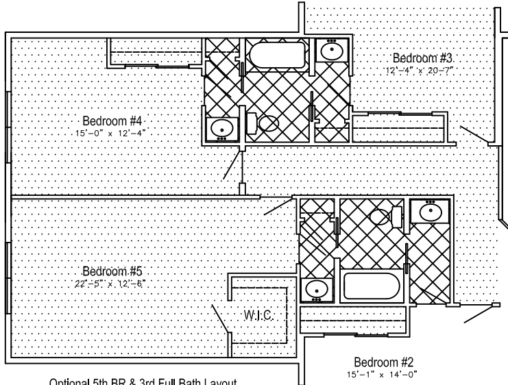
Optional 5th BR & 3rd Full Bath Layout ONLY AVAILABLE WITH 3 CAR SIDELOAD OPTION AND 1ST FLOOR LAUNDRY OPTION
