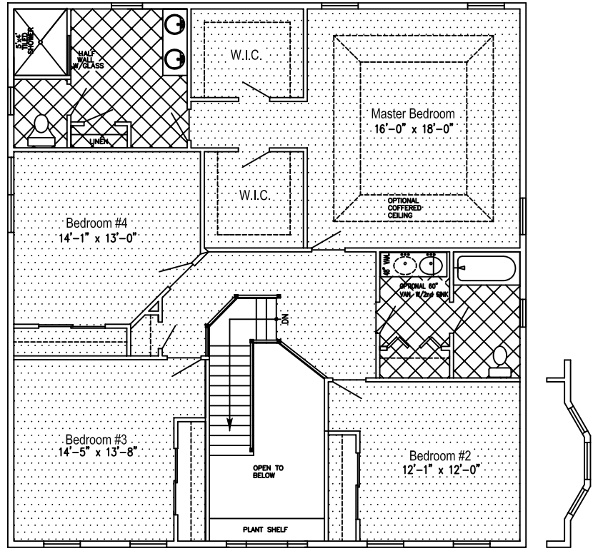
HAWTHORNE SECOND FLOOR
