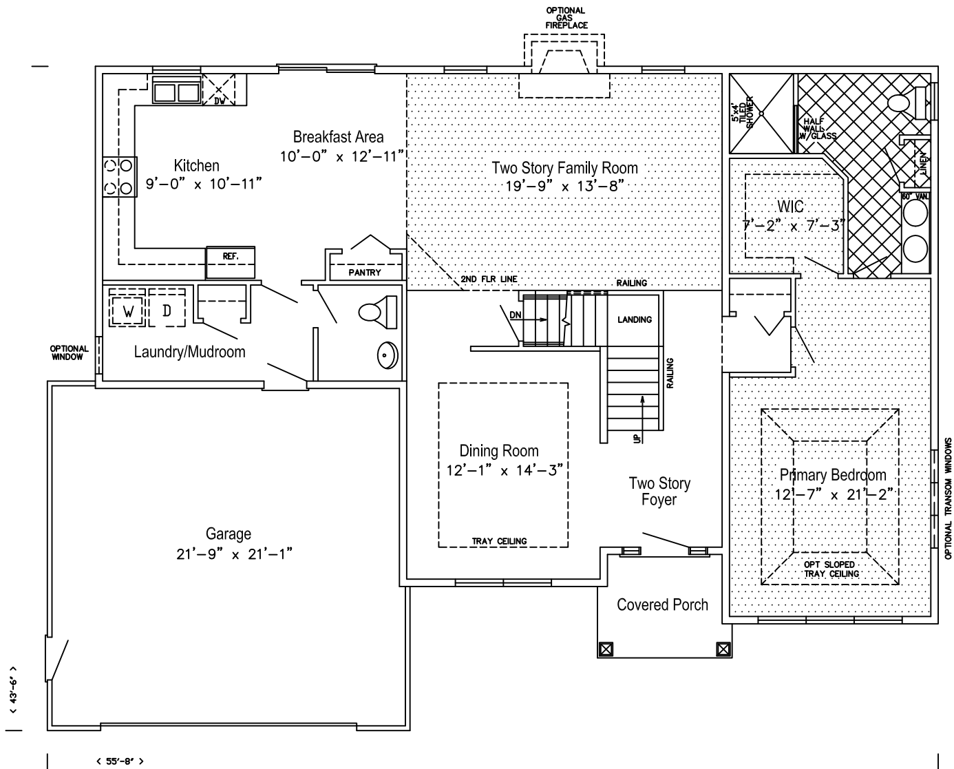
HAMPTON FIRST FLOOR
