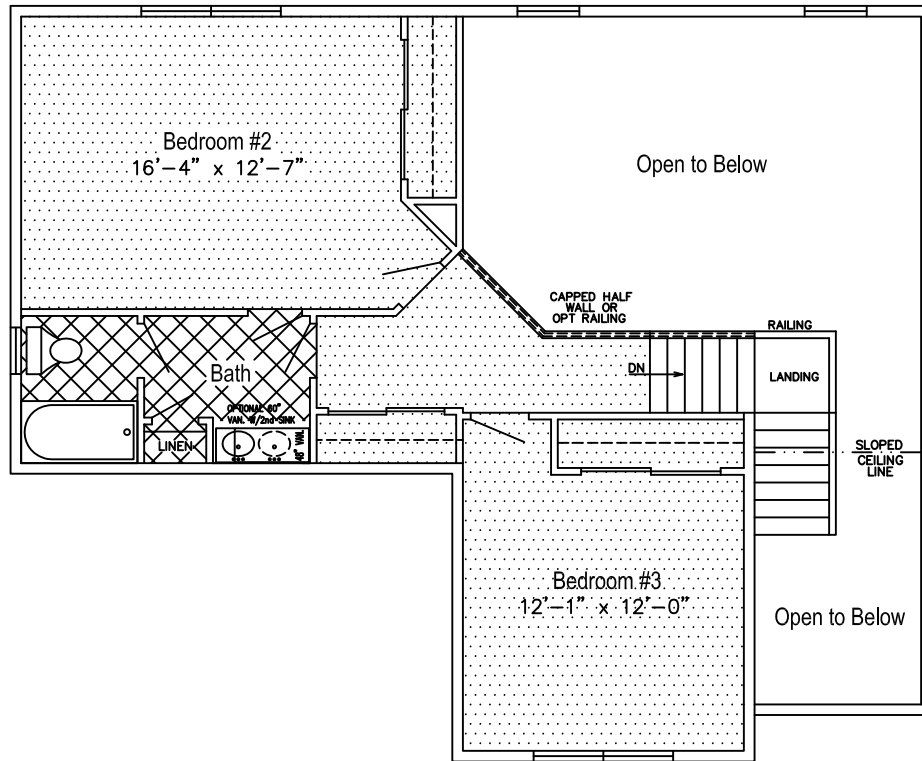
HAMPTON SECOND FLOOR
