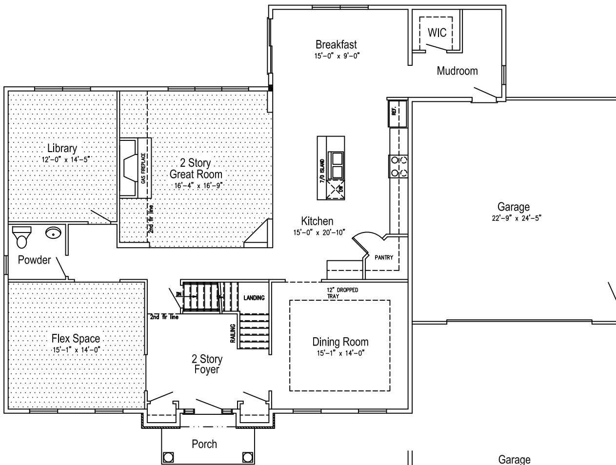
FAULKNER FIRST FLOOR 1885 SQ. FT.
