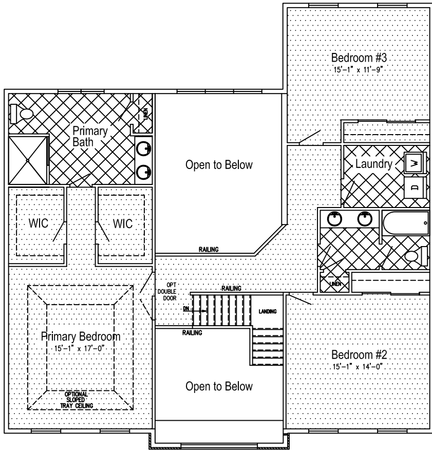
FAULKNER SECOND FLOOR 1373 SQ. FT.
