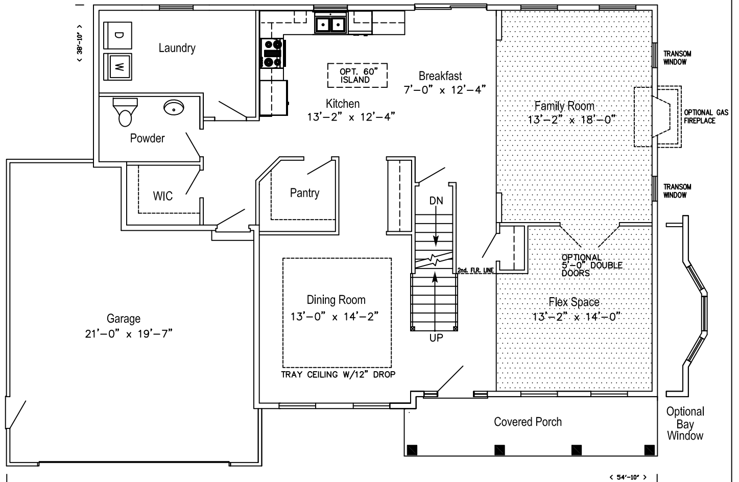
BRENTWOOD FIRST FLOOR
