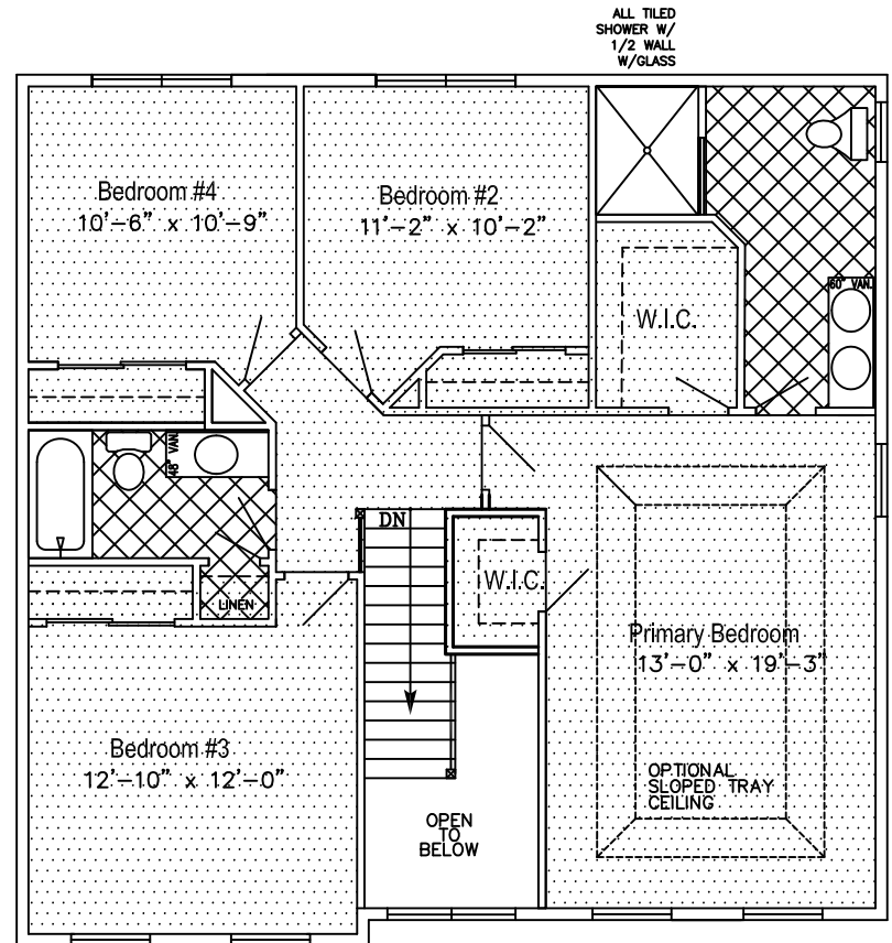
BRENTWOOD SECOND FLOOR
