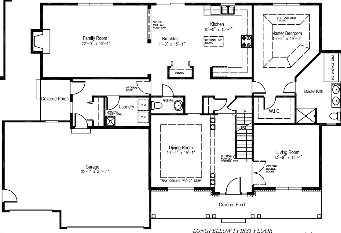
LONGFELLOW I FIRST FLOOR
