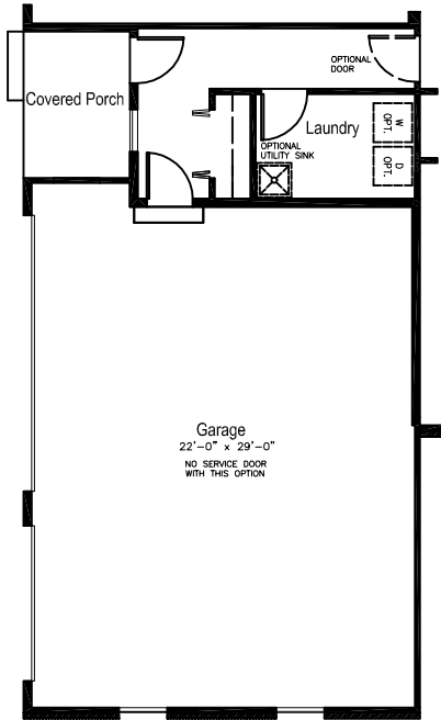
Three Car Side Load Garage Option
